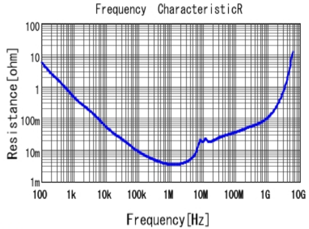
■ GRM21BR71A225MA01 R DCOV, 25degC
