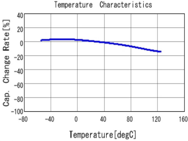
■ GRM21BR71A225MA01 C-Temp. capchange, DC0.0V, AC1.0V r m
