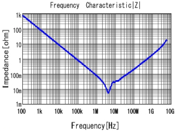
■ GRM21BR71A225MA01 |Z| DCOV, 25degC
