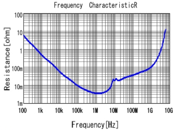
■ GRM21BR71A225KA01 R DCOV, 25degC
