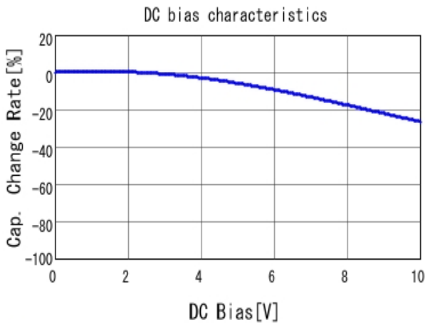
■ GRM21BR71A225KA01 C-DC bias capchange, 25.0degC, AC1.
