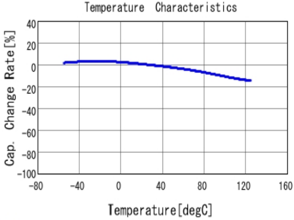
■ GRM21BR71A225KA01 C-Temp. capchange, DC0.0V, AC1.0V r m
