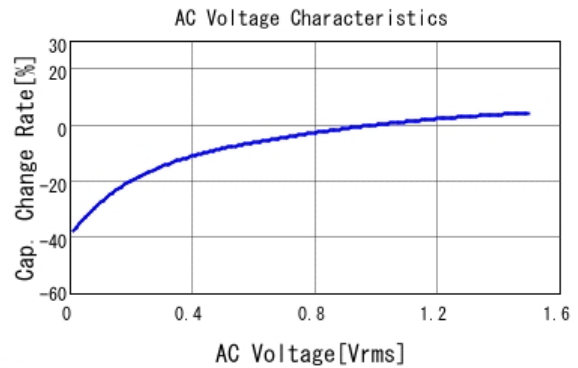
■ GRM21BR71A106MA73 C-AC Voltage capchange, DCOV, 25.0d
