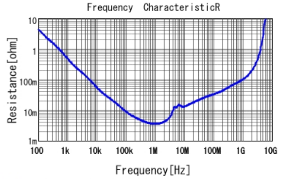
■ GRM21BR71A106MA73 R DCOV, 25degC
