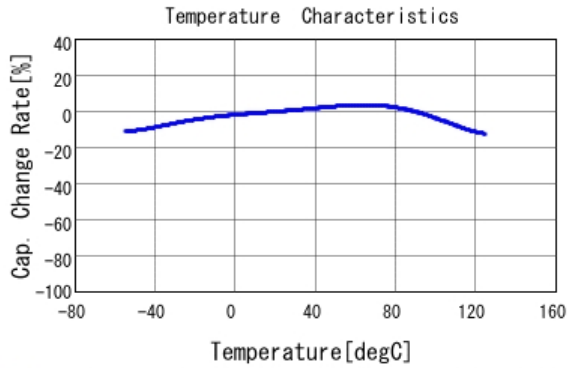
■ GRM21BR71A106MA73 C-Temp. capchange, DC0.0V, AC0.35Vr
