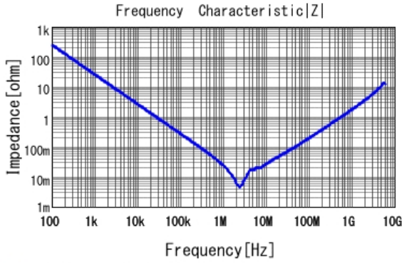
■ GRM21BR71A106MA73 |Z| DCOV, 25degC
