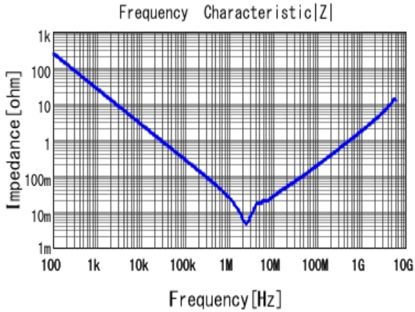
■ GRM21BR71A106KA73 |Z| DCOV, 25degC
