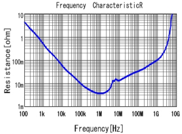
■ GRM21BR71A106KA73 R DCOV, 25degC
