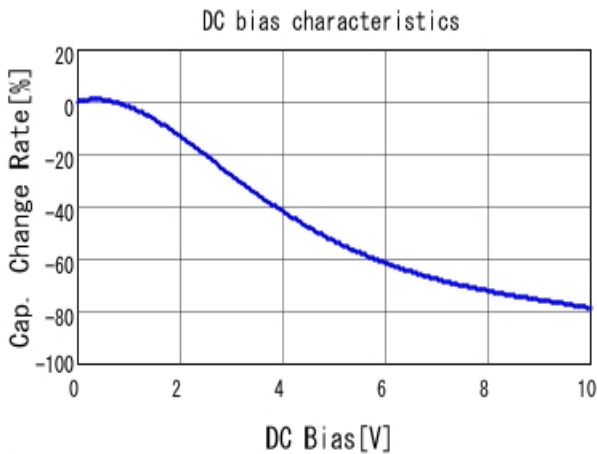
■ GRM21BR71A106KA73 C-DC bias capchange, 25.0degC, AC1V
