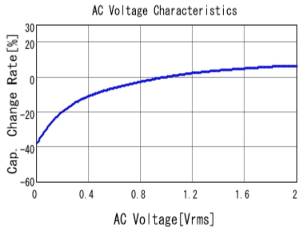
■ GRM21BR71A106KA73 C-AC Voltage capchange, DCOV, 25.0d
