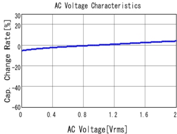
■ GRM21BR71A105KA01 C-AC Voltage capchange, DCOV, 25.0d
