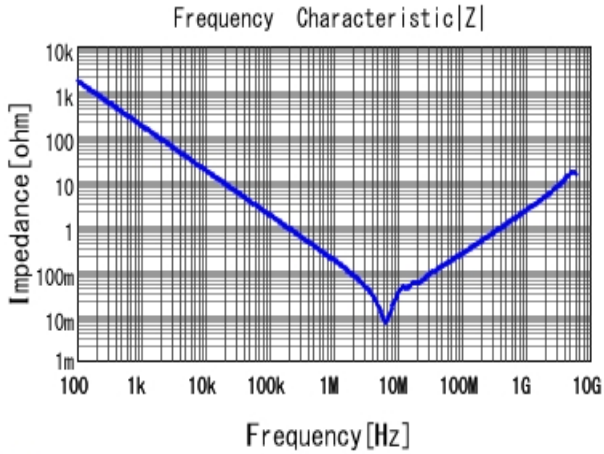
■ GRM21BR71A105KA01 |Z| DCOV, 25degC
