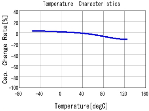
■ GRM21BR71A105KA01 C-Temp. capchange, DC0.0V, AC1.0V rm
