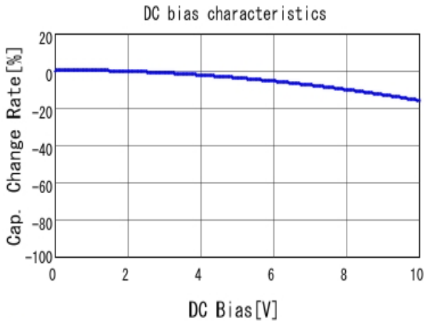
■ GRM21BR71A105KA01 C-DC bias capchange, 25.0degC, AC1.
