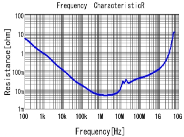
■ GRM21BR71A105KA01 R DCOV, 25degC
