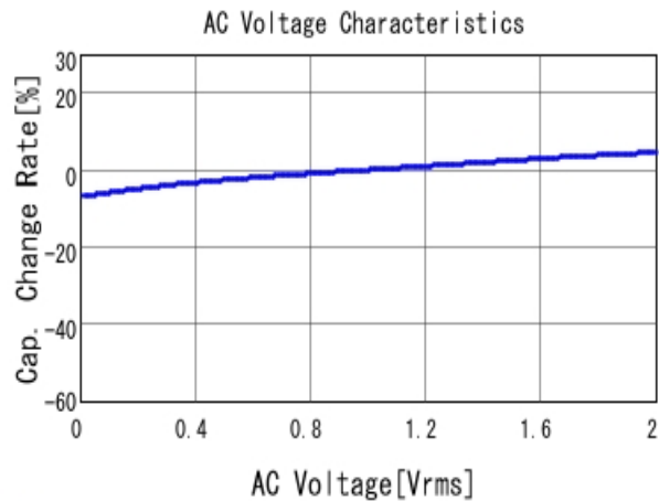
■ GRM21BR70J225KA01 C-AC Voltage capchange, DCOV, 25.0d
