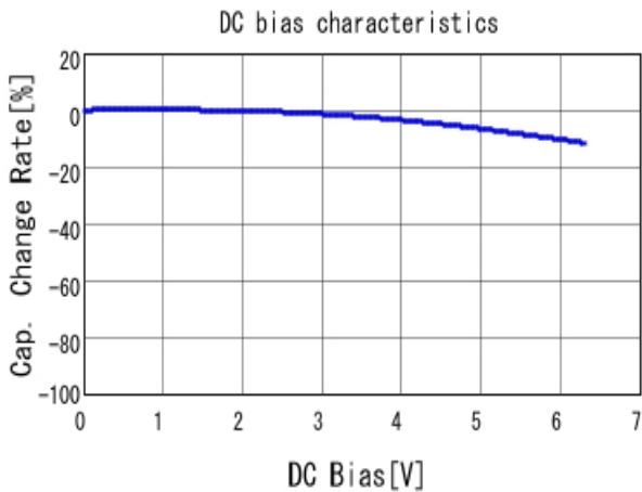
■ GRM21BR70J225KA01 C-DC bias capchange, 25.0degC, AC1.
