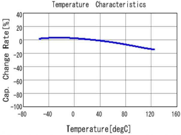
■ GRM21BR70J225KA01 C-Temp. capchange, DC0.0V, AC1.0V r m
