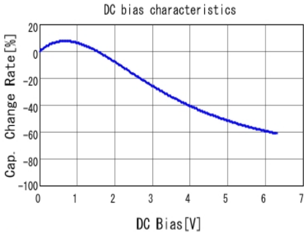
■ GRM21BR70J106KE76 C-DC bias capchange, 25.0degC, AC0.
