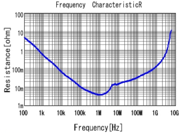
■ GRM21BR70J106KE76 R DCOV, 25degC
