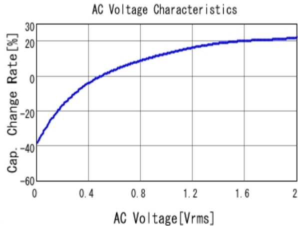
■ GRM21BR70J106KE76 C-AC Voltage capchange, DCOV, 25.0d
