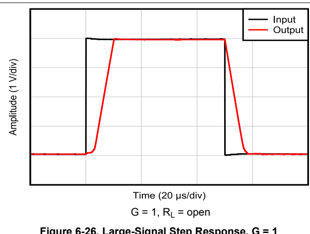
Figure 6-26. Large-Signal Step Response, G = 1
