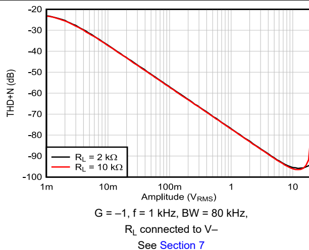
Figure 6-15. THD+N vs Output Amplitude, G = -1
