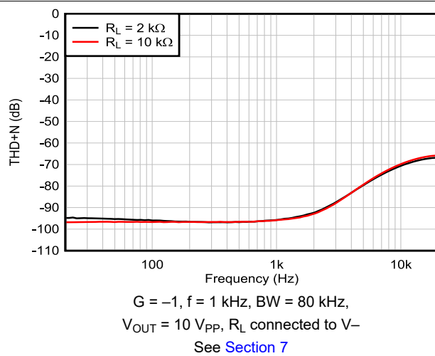
Figure 6-13. THD+N Ratio vs Frequency, G = -1
