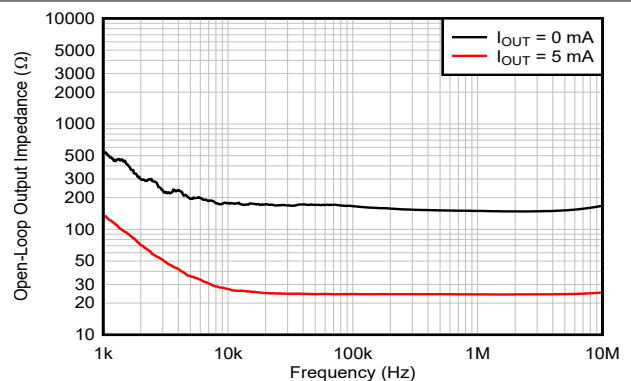
Figure 6-18. Open-Loop Output Impedance vs Frequency
