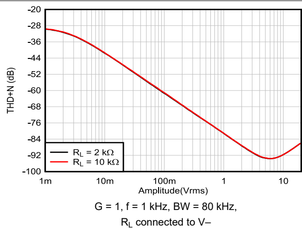
Figure 6-14. THD+N vs Output Amplitude, G = 1
