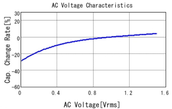
■ GRM21BR6YA106KE43 C-AC Voltage capchange, DCOV, 25.0d
