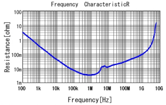
■ GRM21BR6YA106KE43 R DCOV, 25degC
