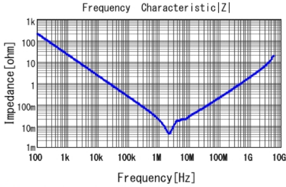
■ GRM21BR6YA106KE43 |Z| DCOV, 25degC
