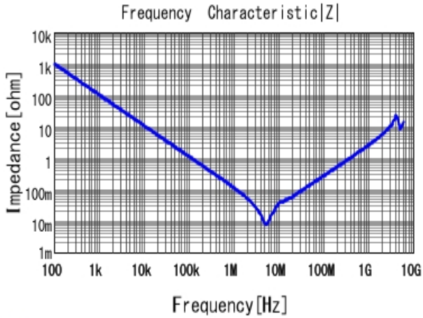
■ GRM21BR61H225KA73 |Z| DCOV, 25degC
