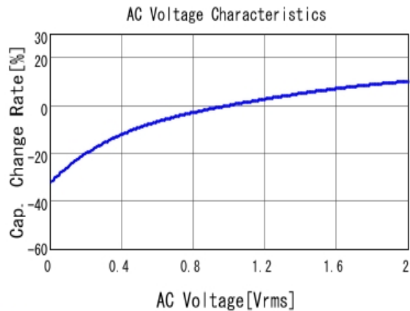
■ GRM21BR61H225KA73 C-AC Voltage capchange, DCOV, 25.0d
