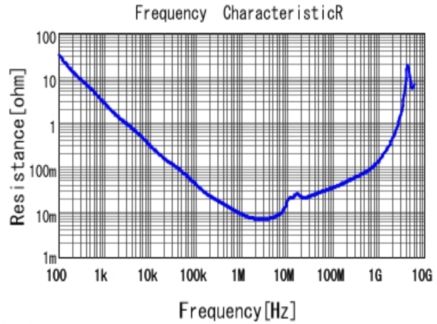
■ GRM21BR61H225KA73 R DCOV, 25degC
