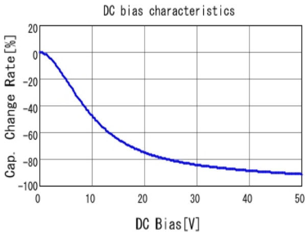
■ GRM21BR61H225KA73 C-DC bias capchange, 25.0degC, AC1.
