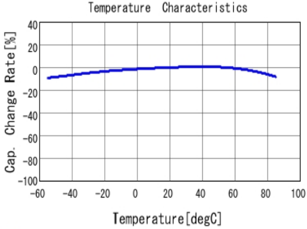
■ GRM21BR61H225KA73 C-Temp. capchange, DC0.0V, AC1.0V rm
