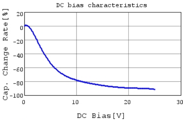
GRM21BR61E226ME44 C-DC bias capchange, 25.0c
