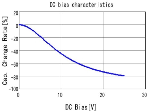
■ GRM21BR61E225KA12 C-DC bias capchange, 25.0degC, AC1.
