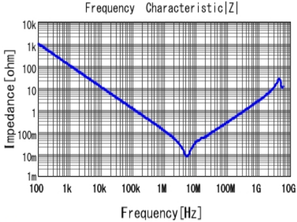
■ GRM21BR61E225KA12 |Z| DCOV, 25degC
