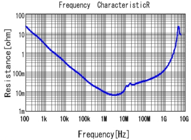
■ GRM21BR61E225KA12 R DCOV, 25degC
