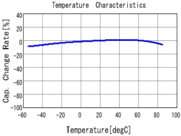
■ GRM21BR61E225KA12 C-Temp. capchange, DC0.0V, AC1.0V rm
