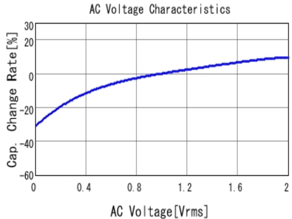
■ GRM21BR61E225KA12 C-AC Voltage capchange, DCOV, 25.0d
