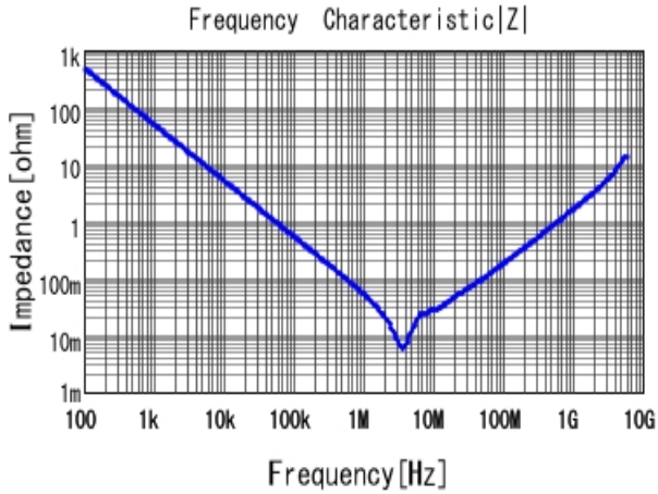
■ GRM21BR61C475KA88 |Z| DCOV, 25degC
