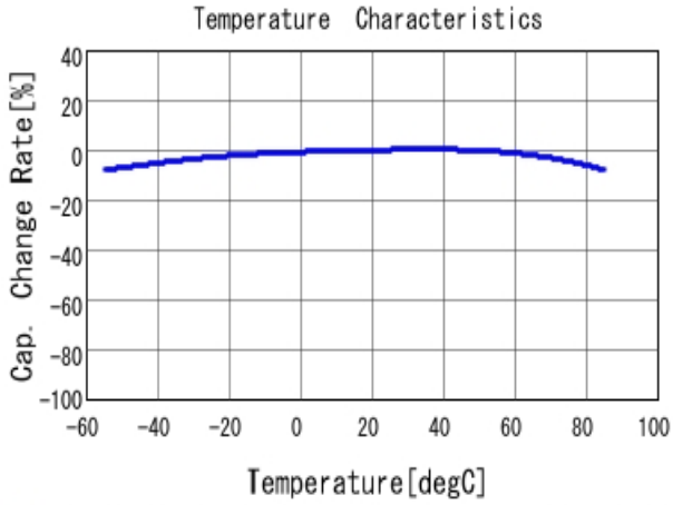
■ GRM21BR61C475KA88 C-Temp. capchange, DC0.0V, AC1.0V r m
