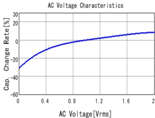
■ GRM21BR61C475KA88 C-AC Voltage capchange, DCOV, 25.0d
