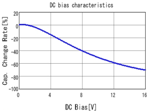
■ GRM21BR61C475KA88 C-DC bias capchange, 25.0degC, AC1.
