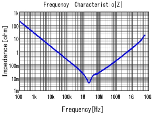
■ GRM21BR61C106KE15 |Z| DCOV, 25degC
