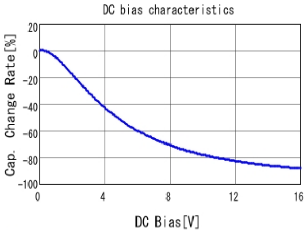
■ GRM21BR61C106KE15 C-DC bias capchange, 25.0degC, AC0.
