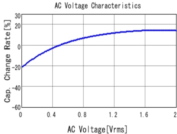
■ GRM21BR61C106KE15 C-AC Voltage capchange, DCOV, 25.0d
