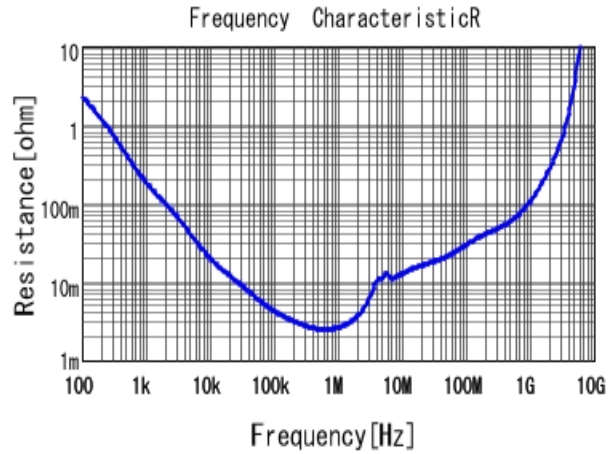
■ GRM21BR61C106KE15 R DCOV, 25degC
