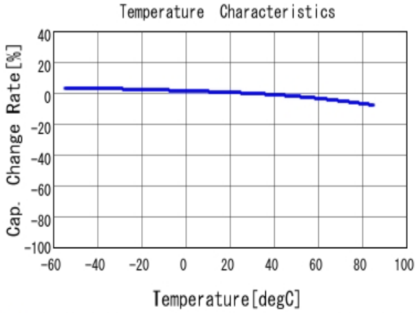
■ GRM21BR61C105KA01 C-Temp. capchange, DC0.0V, AC1.0V rm
