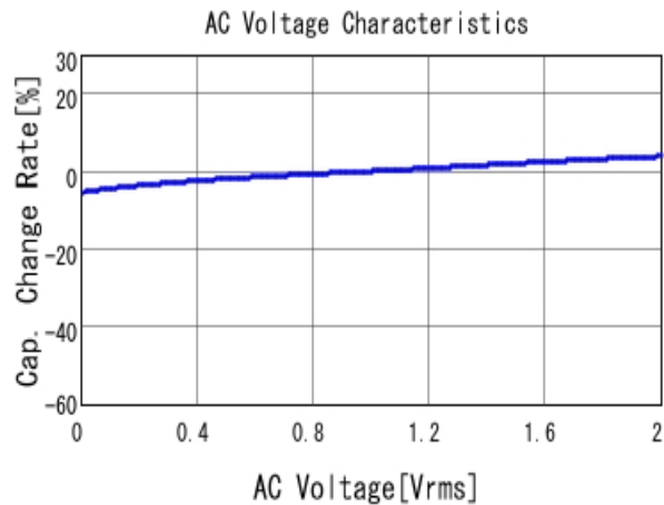
■ GRM21BR61C105KA01 C-AC Voltage capchange, DCOV, 25.0d
