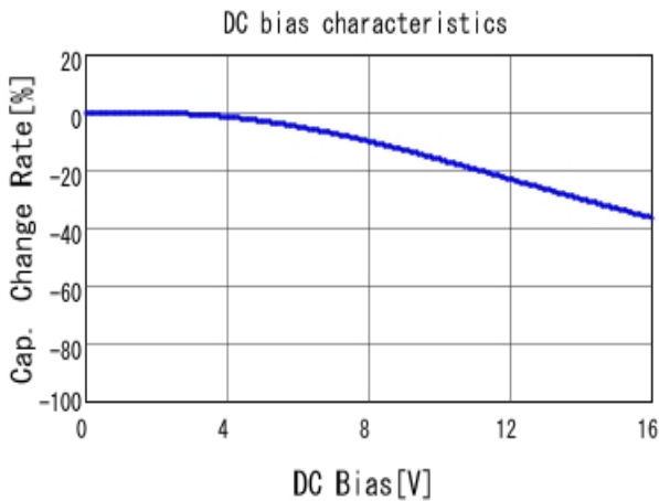
■ GRM21BR61C105KA01 C-DC bias capchange, 25.0degC, AC1.
