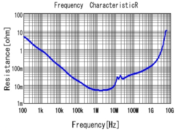
■ GRM21BR61C105KA01 R DCOV, 25degC
