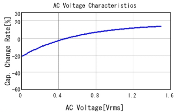
■ GRM21BR61A106KE19 C-AC Voltage capchange, DCOV, 25.0d
