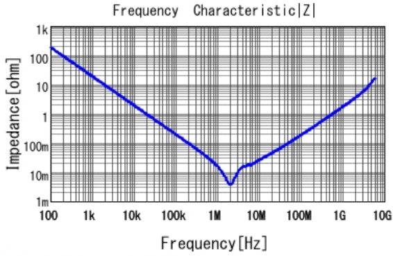
■ GRM21BR61A106KE19 |Z| DCOV, 25degC
