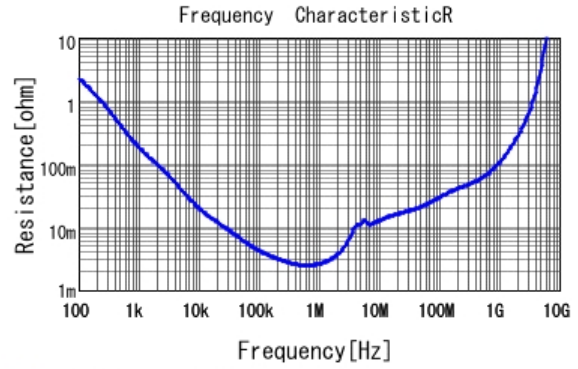
■ GRM21BR61A106KE19 R DCOV, 25degC
