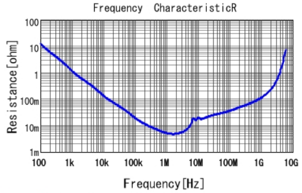
GRM21BR60J475KA11 R DCOV, 25degC
