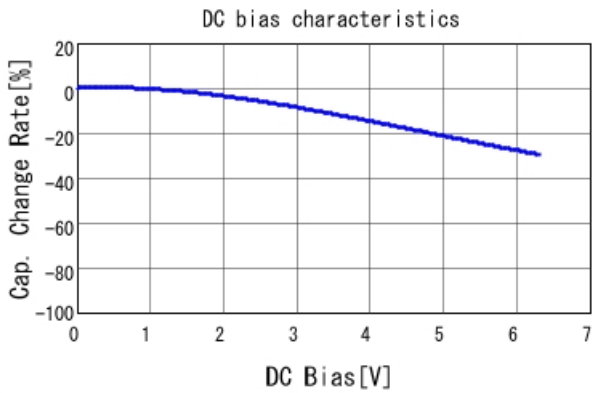
GRM21BR60J475KA11 C-DC bias capchange, 25.0degC, A
