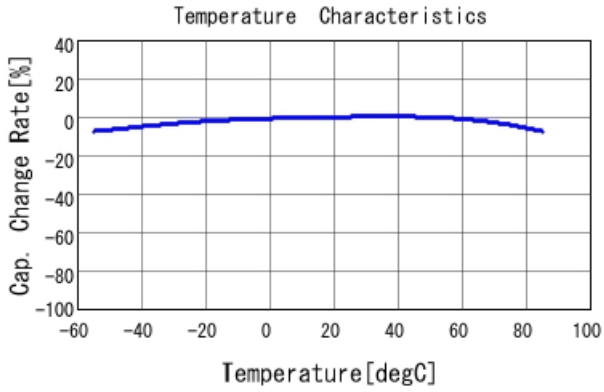
GRM21BR60J475KA11 C-Temp. capchange, DC0.0V, AC1.C
