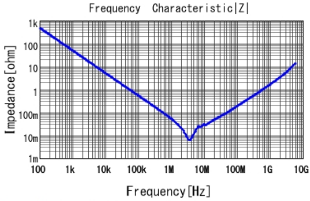
GRM21BR60J475KA11 |Z| DCOV, 25degC
