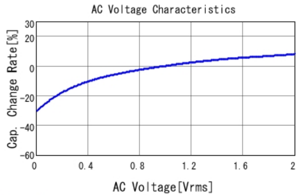
GRM21BR60J475KA11 C-AC Voltage capchange, DCOV, 25
