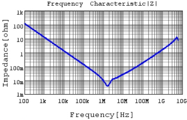
GRM21BR60J226ME39 |Z| DCOV, 25degC
