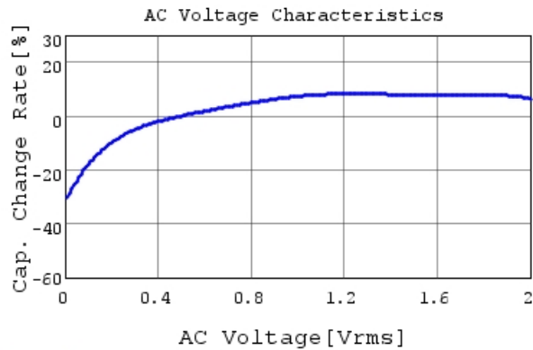
GRM21BR60J226ME39 C-AC Voltage capchange, Dc
