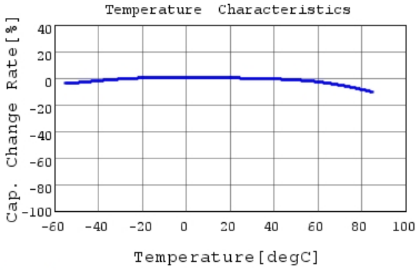
GRM21BR60J226ME39 C-Temp. capchange, DC0.0V,
