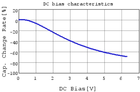
GRM21BR60J226ME39 C-DC bias capchange, 25.0c
