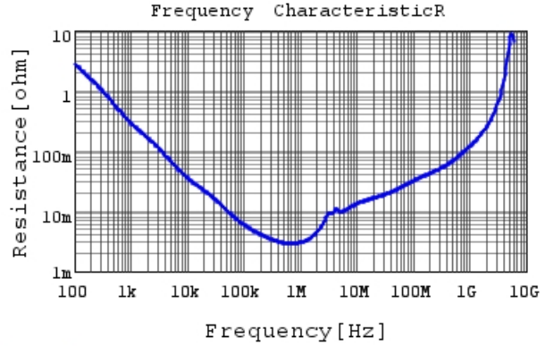
GRM21BR60J226ME39 R DCOV, 25degC
