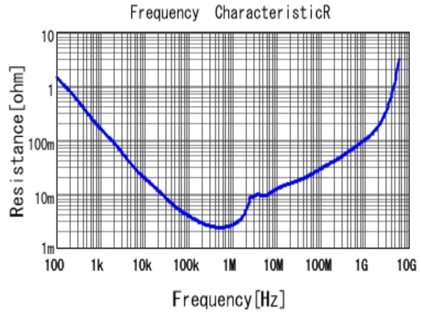
■ GRM21BD71A226ME44 R DCOV, 25degC
