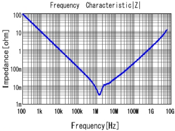
■ GRM21BD71A226ME44 |Z| DCOV, 25degC
