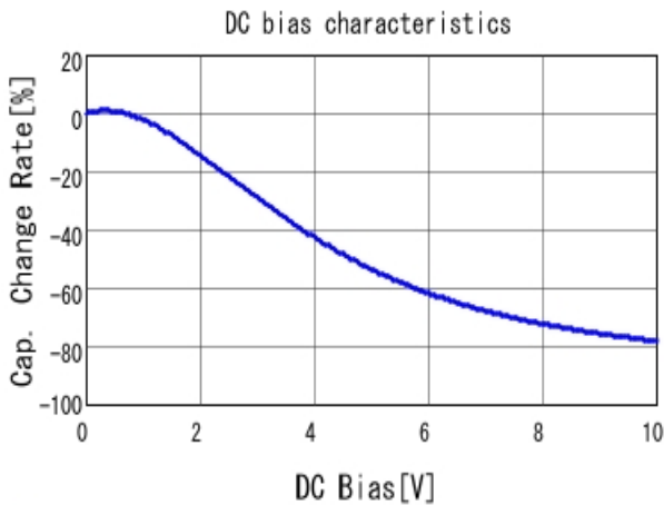
■ GRM21BD71A226ME44 C-DC bias capchange, 25.0degC, AC0.
