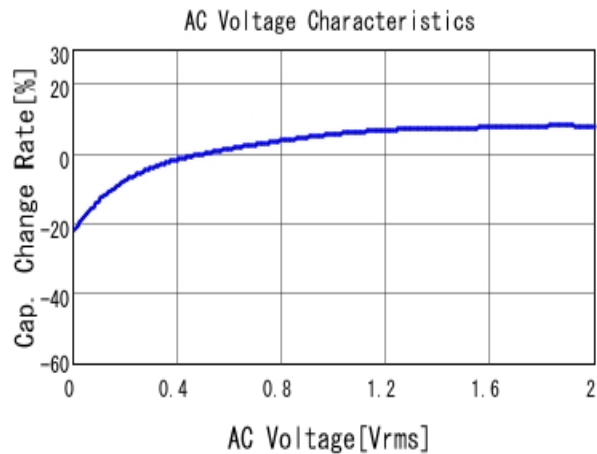
■ GRM21BD71A226ME44 C-AC Voltage capchange, DCOV, 25.0d
