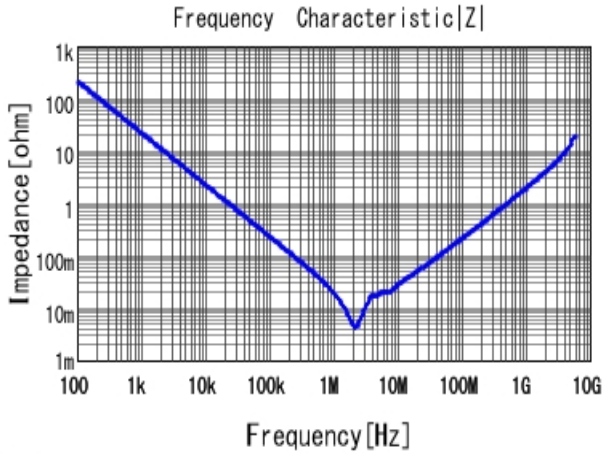
■ GRM21BC8YA106KE11 |Z| DCOV, 25degC
