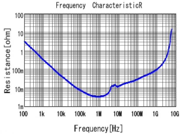
■ GRM21BC8YA106KE11 R DCOV, 25degC
