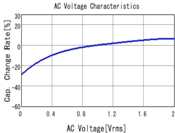
■ GRM21BC8YA106KE11 C-AC Voltage capchange, DCOV, 25.0d
