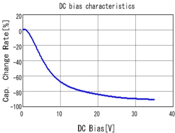
■ GRM21BC8YA106KE11 C-DC bias capchange, 25.0degC, AC1V
