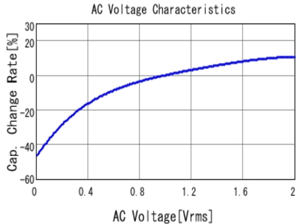
■ GRM21BC81E106KE51 C-AC Voltage capchange, DCOV, 25.0d
