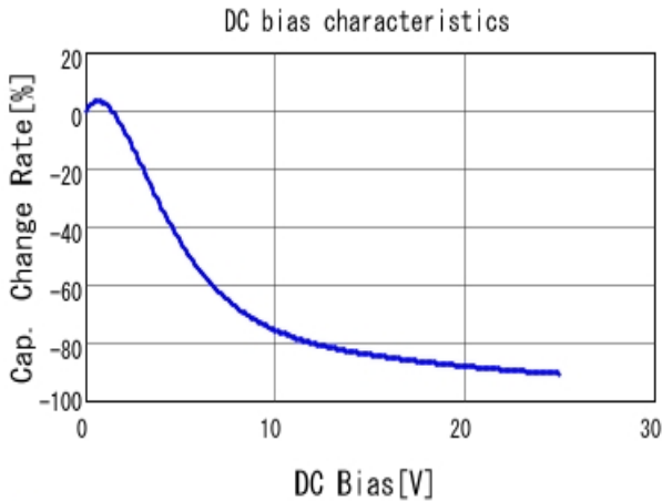
■ GRM21BC81E106KE51 C-DC bias capchange, 25.0degC, AC1.
