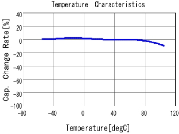
■ GRM21BC81E106KE51 C-Temp. capchange, DC0.0V, AC1.0V r m
