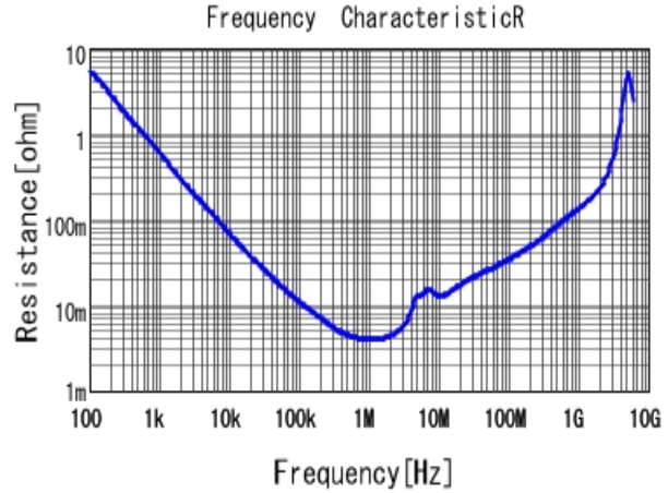
■ GRM21BC81E106KE51 R DCOV, 25degC
