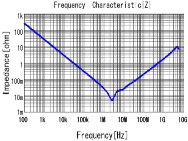
■ GRM21BC81E106KE51 |Z| DCOV, 25degC
