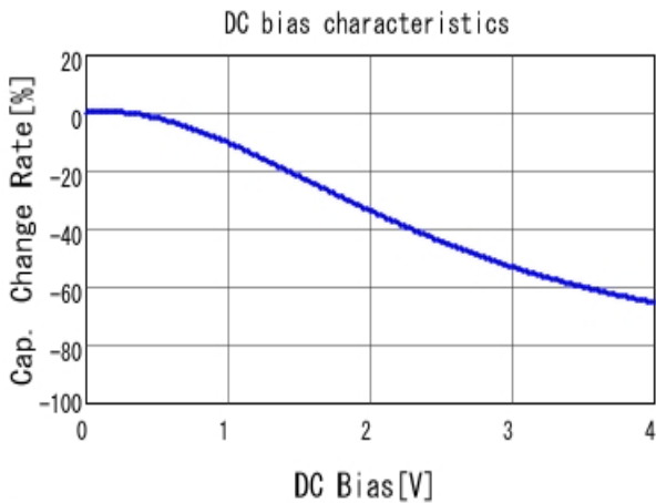
■ GRM21BC80G476ME15 C-DC bias capchange, 25.0degC, AC0.
