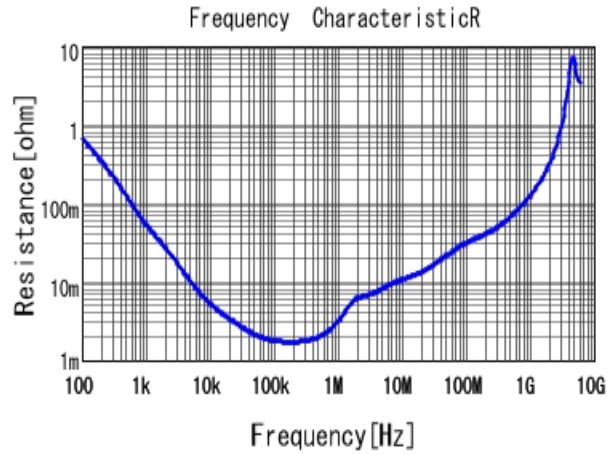
■ GRM21BC80G476ME15 R DCOV, 25degC
