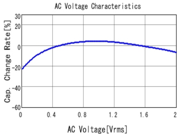
■ GRM21BC80G476ME15 C-AC Voltage capchange, DCOV, 25.0d
