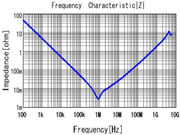
■ GRM21BC80G476ME15 |Z| DCOV, 25degC
