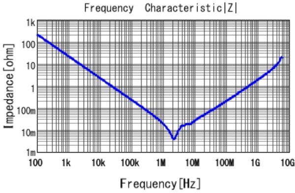
■ GRM21BC71E106ME11 |Z| DCOV, 25degC
