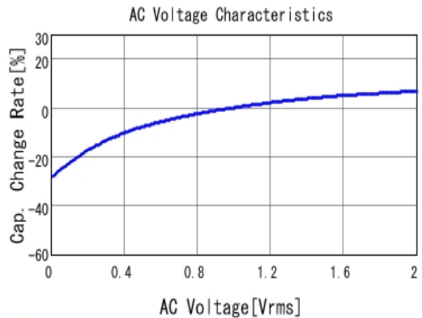
■ GRM21BC71E106KE11 C-AC Voltage capchange, DCOV, 25.0d
