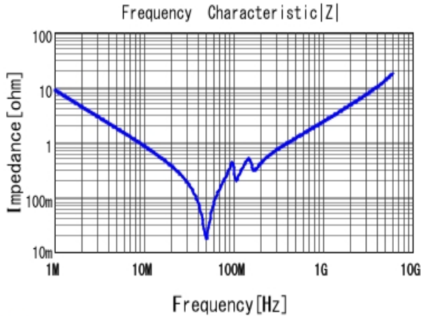
■ GRM21B5C1H183JA01 |Z| DC0V, 25degC
