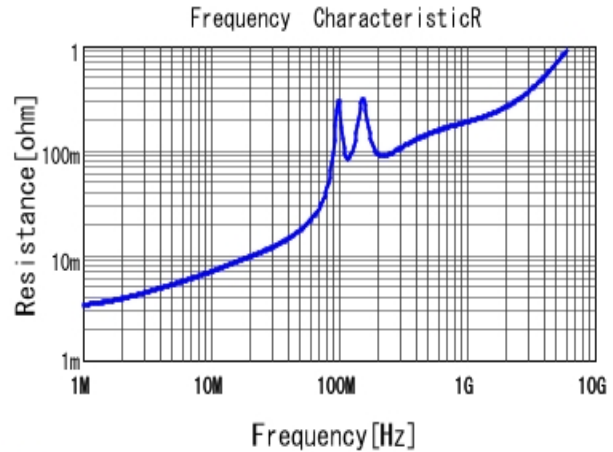
■ GRM21B5C1H183JA01 R DC0V, 25degC
