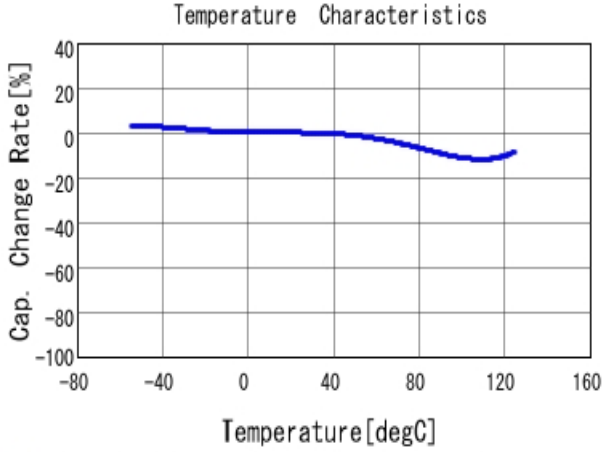
■ GRM21AR72E102KW01 C-Temp. capchange, DCOV, AC1Vrms
