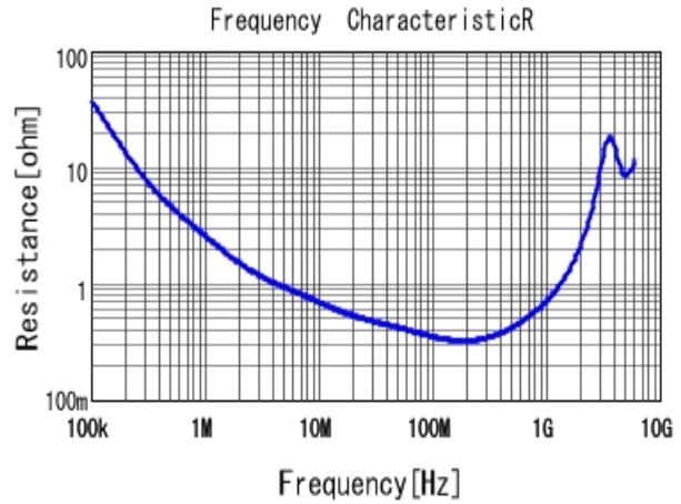
■ GRM21AR72E102KW01 R DCOV, 25degC
