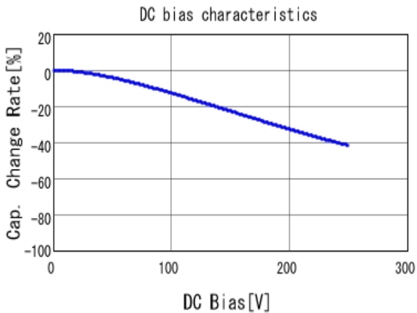
■ GRM21AR72E102KW01 C-DC bias capchange, 25.0degC, AC1V
