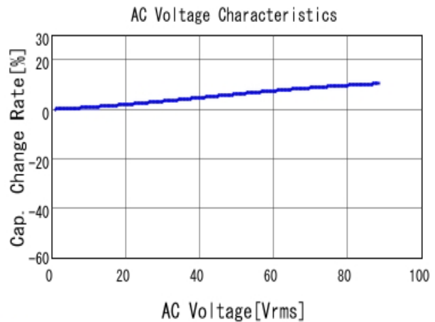
■ GRM21AR72E102KW01 C-AC Voltage capchange, DCOV, 25.0d
