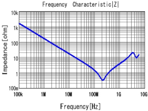
■ GRM21AR72E102KW01 |Z| DCOV, 25degC
