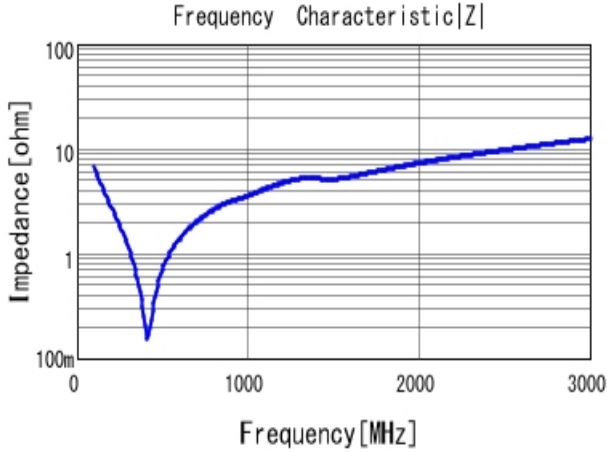
■ GRM21A7U2E221JW31 |Z| DCOV, 25degC
