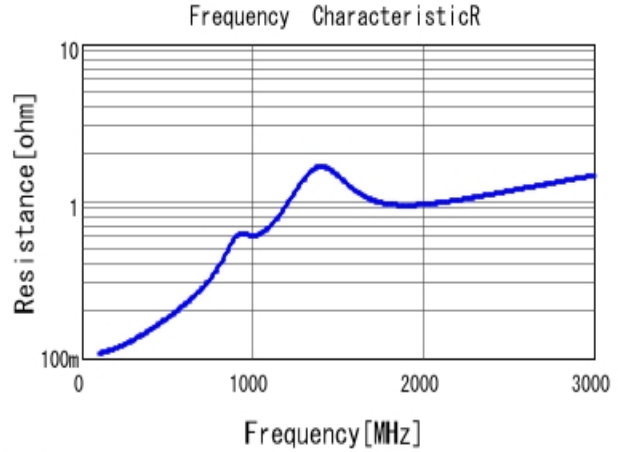
■ GRM21A7U2E221JW31 R DCOV, 25degC
