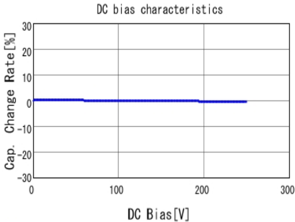
■ GRM21A7U2E221JW31 C-DC bias capchange, 25.0degC, AC1V
