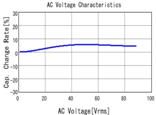
■ GRM21A7U2E221JW31 C-AC Voltage capchange, DCOV, 25.0d
