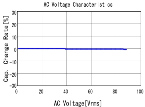
■ GRM21A7U2E102JW31 C-AC Voltage capchange, DCOV, 25.0d
