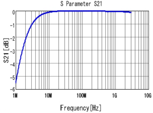
■ GRM21A7U2E102JW31 S21 DCOV, 25degC
