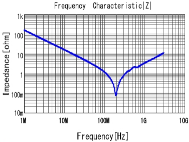
■ GRM21A7U2E102JW31 |Z| DCOV, 25degC
