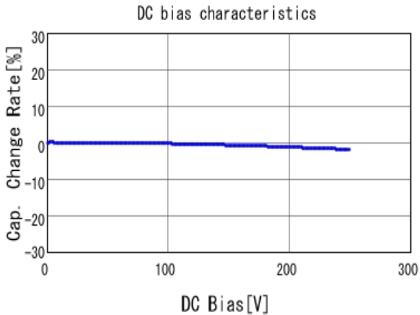
■ GRM21A7U2E102JW31 C-DC bias capchange, 25.0degC, AC1V
