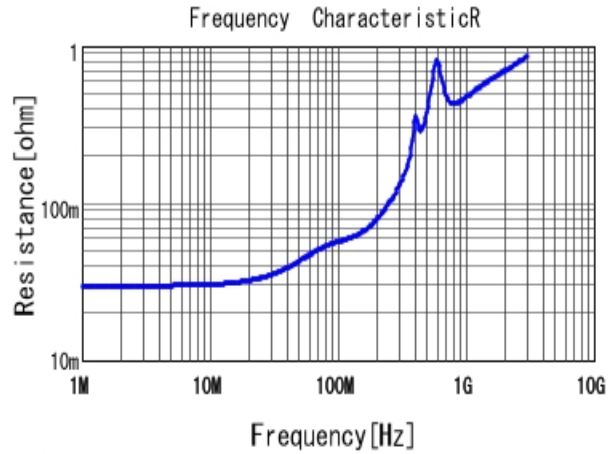
■ GRM21A7U2E102JW31 R DCOV, 25degC
