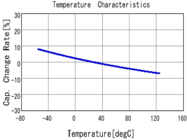
■ GRM21A7U2E102JW31 C-Temp. capchange, DCOV, AC1Vrms
