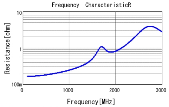
■ GRM21A5C2E820JW01 R DC0V, 25degC
