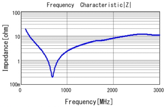
■ GRM21A5C2E820JW01 |Z| DC0V, 25degC
