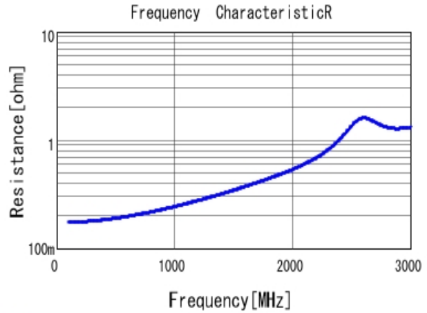
■ GRM21A5C2E390JW01 R DCOV, 25degC
