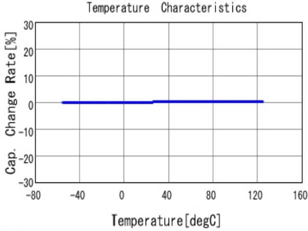
■ GRM21A5C2E390JW01 C-Temp. capchange, DCOV, AC1Vrms
