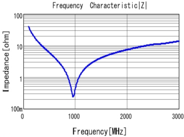
■ GRM21A5C2E390JW01 |Z| DCOV, 25degC
