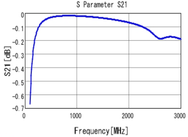
■ GRM21A5C2E390JW01 S21 DCOV, 25degC
