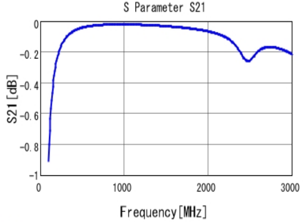
■ GRM21A5C2E330JW01 S21 DCOV, 25degC
