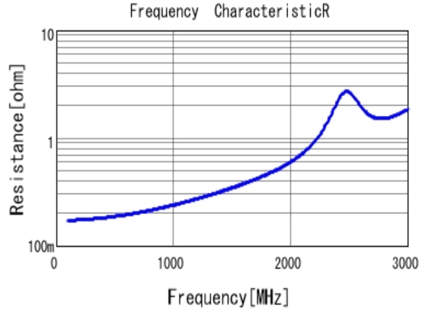
■ GRM21A5C2E330JW01 R DC0V, 25degC
