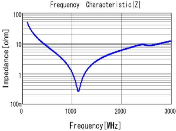
■ GRM21A5C2E330JW01 |Z| DC0V, 25degC
