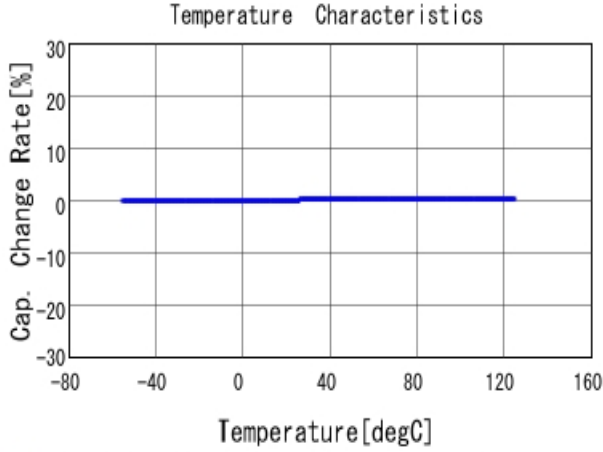
■ GRM21A5C2E330JW01 C-Temp. capchange, DCOV, AC1Vrms
