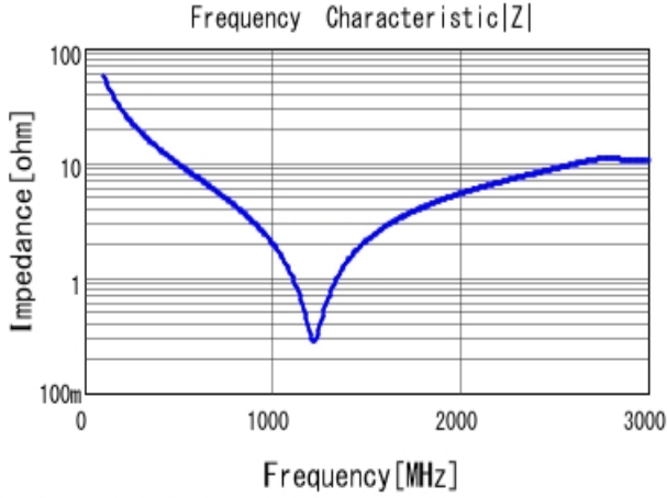
■ GRM21A5C2E270JW01 |Z| DCOV, 25degC
