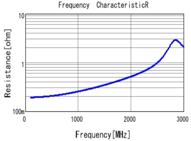
■ GRM21A5C2E270JW01 R DCOV, 25degC
