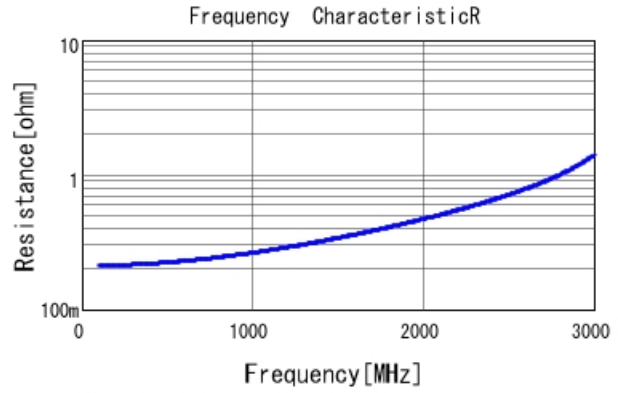
GRM21A5C2E220JW01 R DCOV, 25degC
