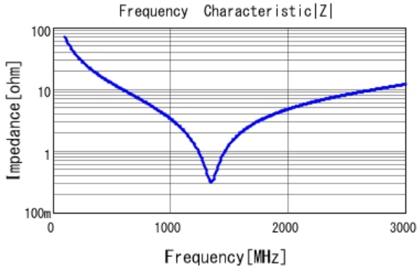
GRM21A5C2E220JW01 |Z| DCOV, 25degC
