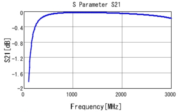
GRM21A5C2E220JW01 S21 DCOV, 25degC
