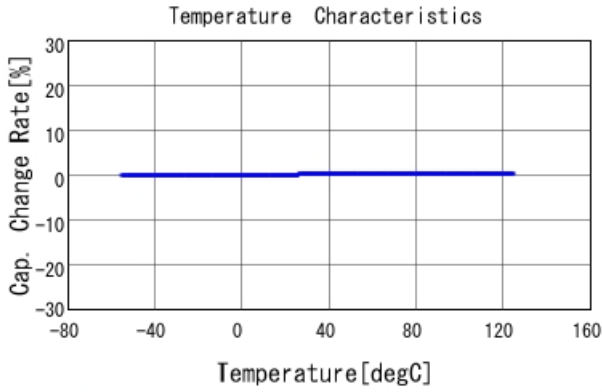
GRM21A5C2E220JW01 C-Temp. capchange, DCOV, AC1Vrms
