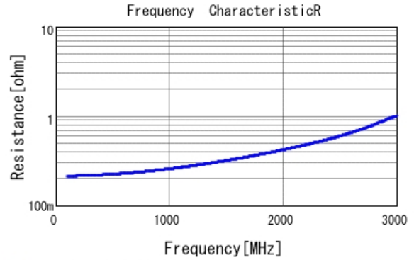
■ GRM21A5C2E180JW01 R DC0V, 25degC
