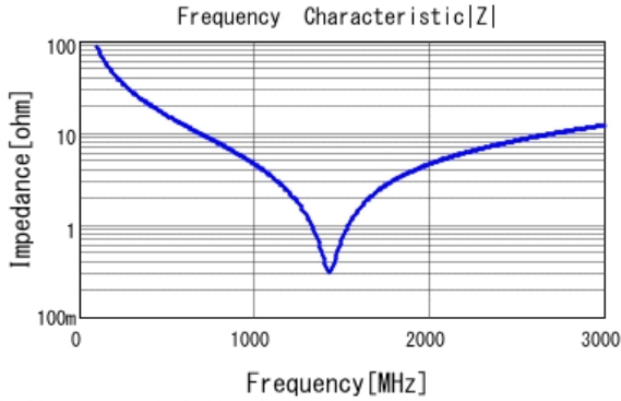
■ GRM21A5C2E180JW01 |Z| DC0V, 25degC
