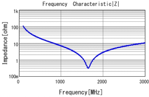
■ GRM21A5C2E150JW01 |Z| DC0V, 25degC
