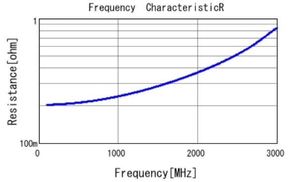
■ GRM21A5C2E150JW01 R DC0V, 25degC
