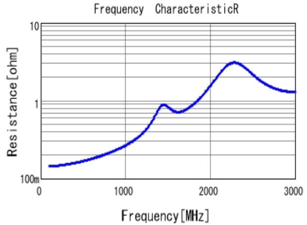
■ GRM21A5C2E101JW01 R DCOV, 25degC
