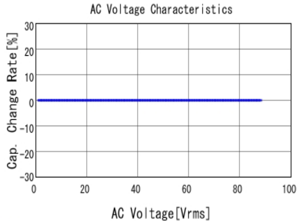
■ GRM21A5C2E101JW01 C-AC Voltage capchange, DCOV, 25.0d
