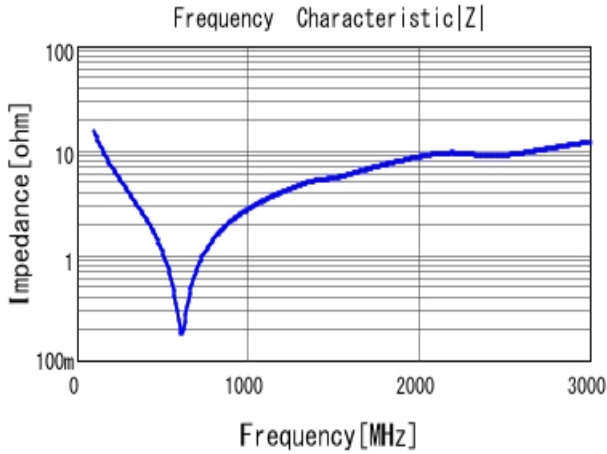
■ GRM21A5C2E101JW01 |Z| DCOV, 25degC
