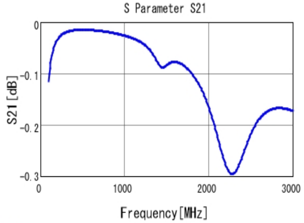
■ GRM21A5C2E101JW01 S21 DCOV, 25degC
