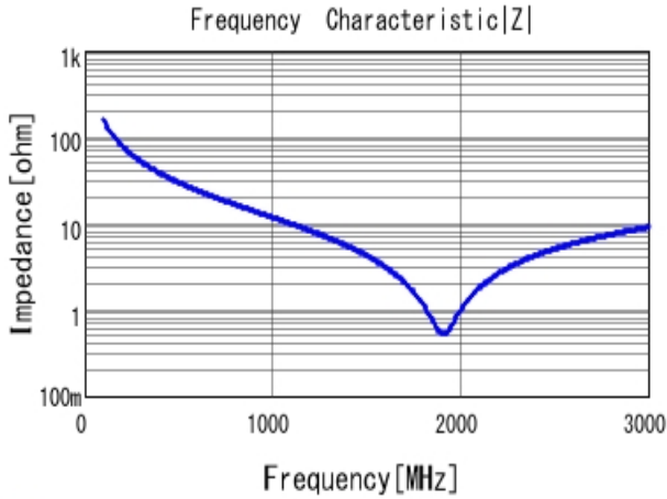
■ GRM21A5C2E100JW01 |Z| DC0V, 25degC
