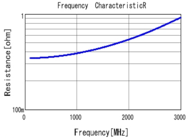
■ GRM21A5C2E100JW01 R DC0V, 25degC
