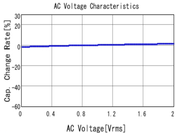
■ GRM219R72A682KA01 C-AC Voltage capchange, DCOV, 25.0d
