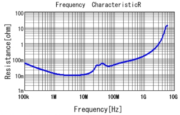
■ GRM219R71H334KA88 R DCOV, 25degC
