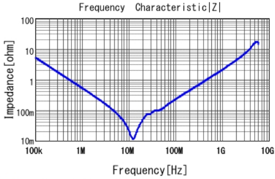
■ GRM219R71H334KA88 |Z| DCOV, 25degC
