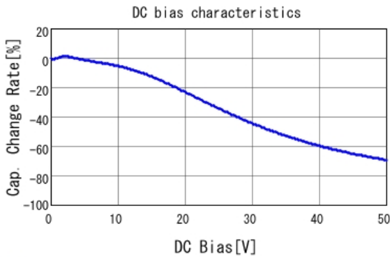
■ GRM219R71H334KA88 C-DC bias capchange, 25.0degC, AC1.
