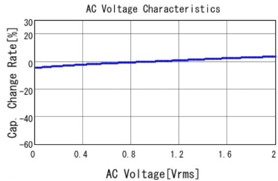
■ GRM219R71H334KA88 C-AC Voltage capchange, DCOV, 25.0d
