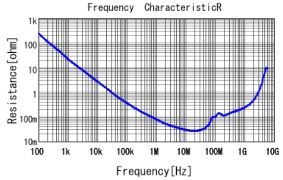
■ GRM219R71H333KA01 R DCOV, 25degC
