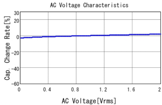
■ GRM219R71H333KA01 C-AC Voltage capchange, DCOV, 25.0d
