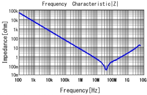
■ GRM219R71H333KA01 |Z| DCOV, 25degC
