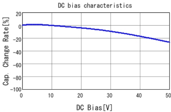
■ GRM219R71H333KA01 C-DC bias capchange, 25.0degC, AC1.
