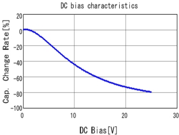
■ GRM219R61E225KA12 C-DC bias capchange, 25.0degC, AC1.
