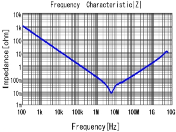
■ GRM219R61E225KA12 |Z| DCOV, 25degC
