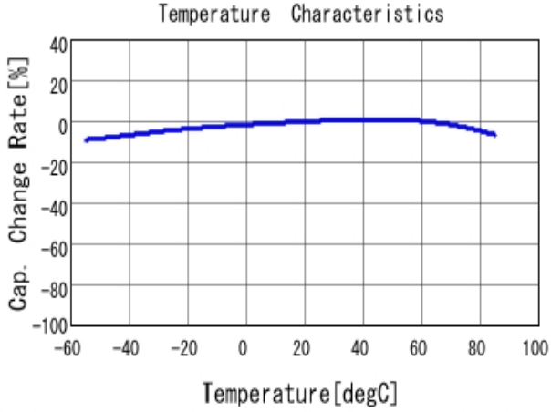
■ GRM219R61E225KA12 C-Temp. capchange, DC0.0V, AC1.0V rm
