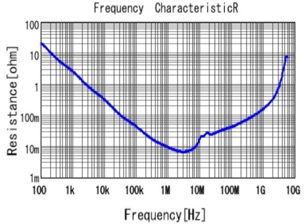
■ GRM219R61E225KA12 R DCOV, 25degC
