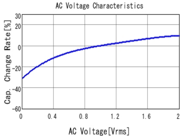
■ GRM219R61E225KA12 C-AC Voltage capchange, DCOV, 25.0d
