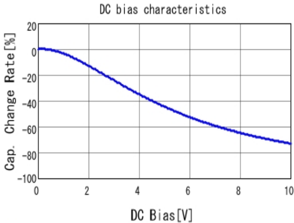
■ GRM219R61A106KE44 C-DC bias capchange, 25.0degC, AC0.
