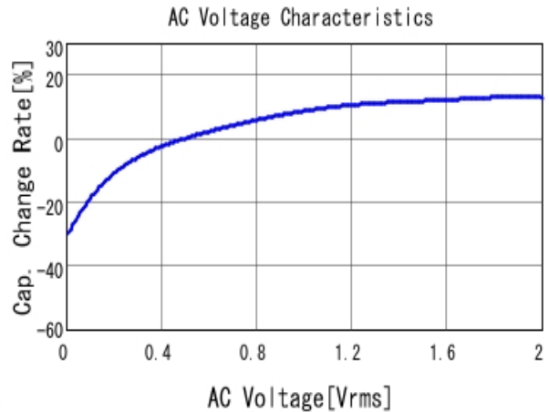
■ GRM219R61A106KE44 C-AC Voltage capchange, DCOV, 25.0d
