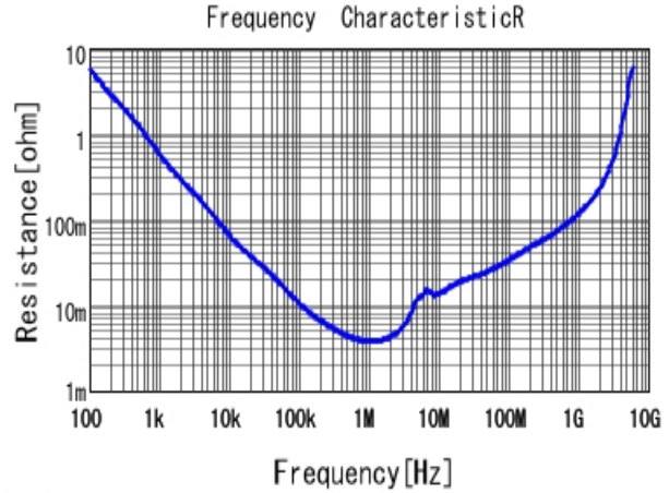
■ GRM219R61A106KE44 R DCOV, 25degC
