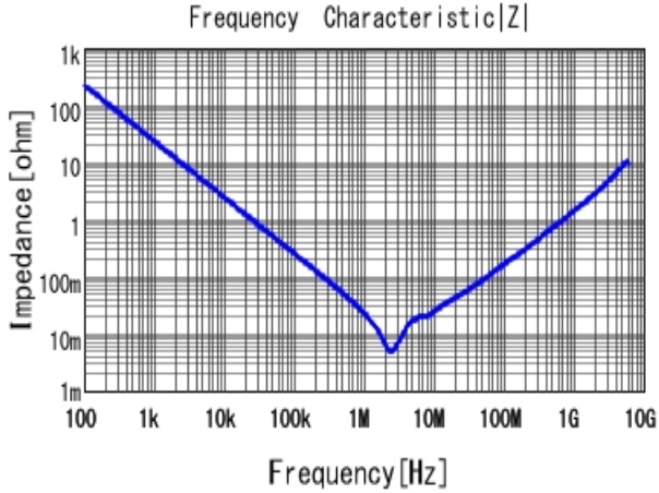
■ GRM219R61A106KE44 |Z| DCOV, 25degC
