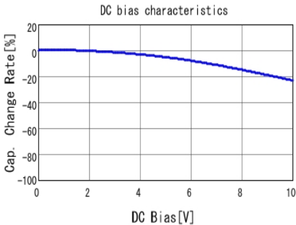
■ GRM219R61A105KA01 C-DC bias capchange, 25.0degC, AC1.
