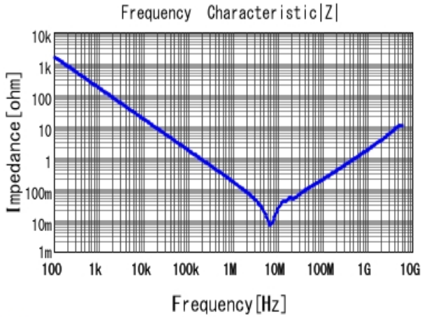
■ GRM219R61A105KA01 |Z| DCOV, 25degC
