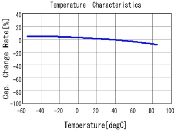
■ GRM219R61A105KA01 C-Temp. capchange, DC0.0V, AC1.0V rm
