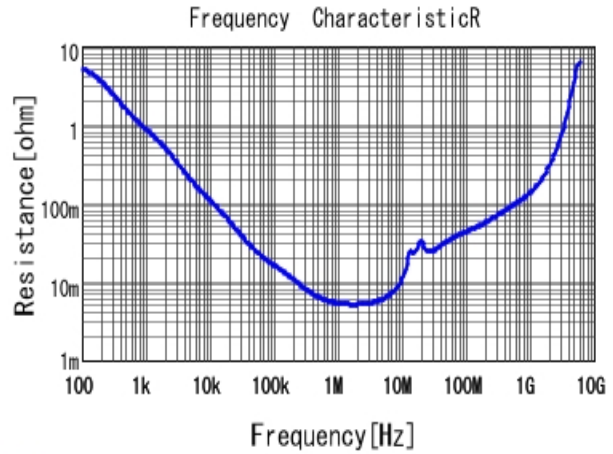
■ GRM219R61A105KA01 R DCOV, 25degC
