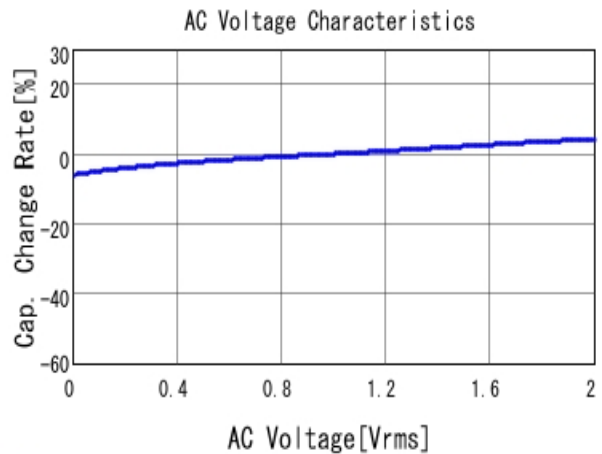
■ GRM219R61A105KA01 C-AC Voltage capchange, DCOV, 25.0d
