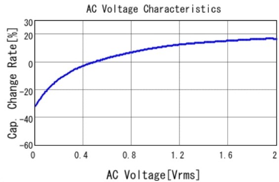
■ GRM219R60J475KE19 C-AC Voltage capchange, DCOV, 25.0d
