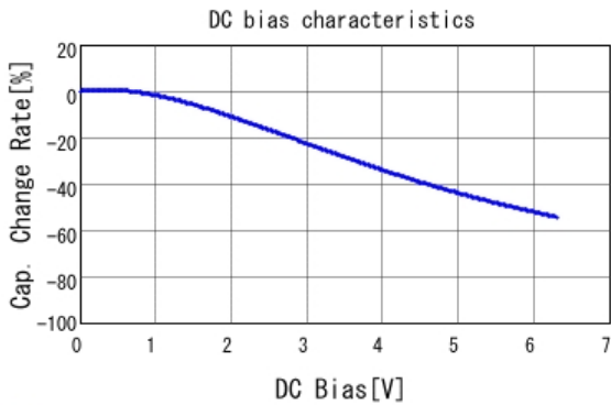
■ GRM219R60J475KE19 C-DC bias capchange, 25.0degC, AC0.
