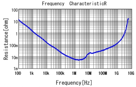
■ GRM219R60J475KE19 R DCOV, 25degC
