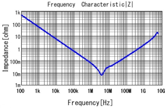
■ GRM219R60J475KE19 |Z| DCOV, 25degC
