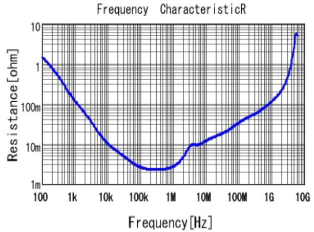
■ GRM219R60J226ME47 R DCOV, 25degC
