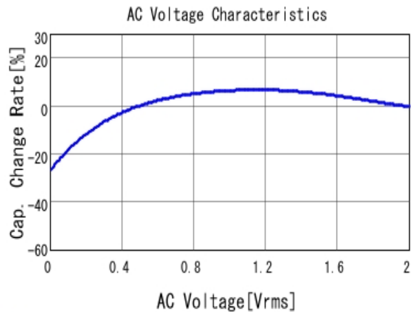
■ GRM219R60J226ME47 C-AC Voltage capchange, DCOV, 25.0d
