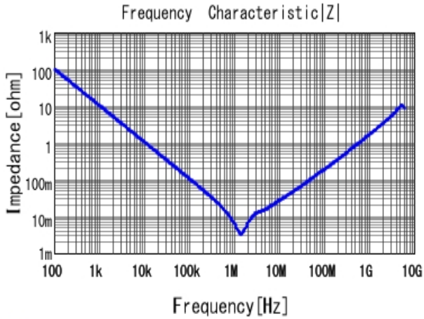
■ GRM219R60J226ME47 |Z| DCOV, 25degC
