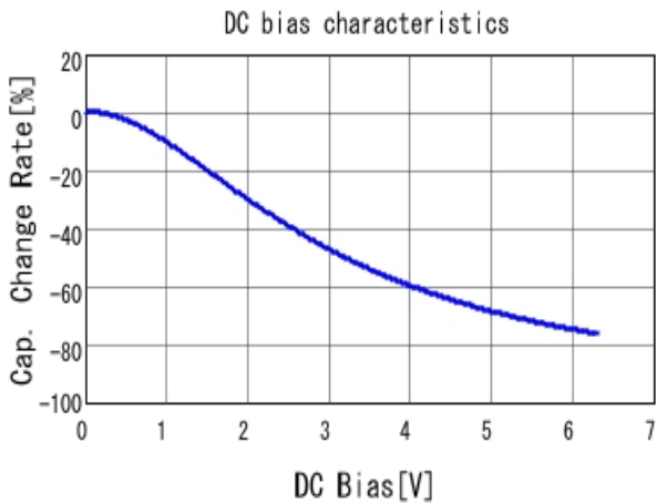
■ GRM219R60J226ME47 C-DC bias capchange, 25.0degC, AC0.
