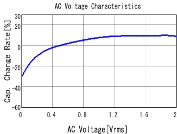
■ GRM219R60J106KE19 C-AC Voltage capchange, DCOV, 25.0d
