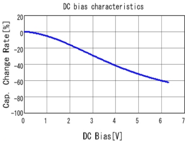
■ GRM219R60J106KE19 C-DC bias capchange, 25.0degC, AC0.
