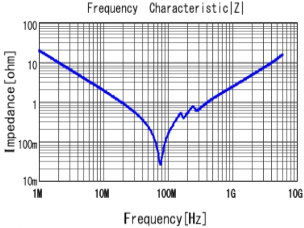
■ GRM2195C1H822JA01 |Z| DCOV, 25degC
