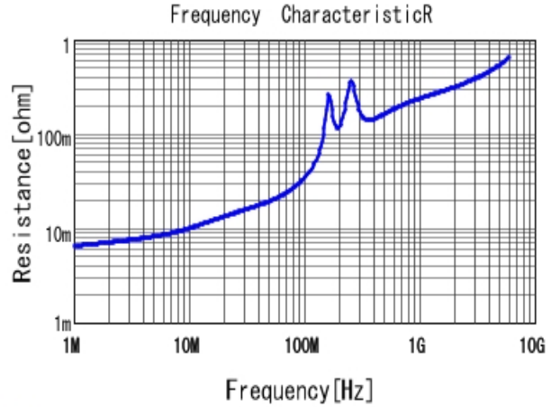
■ GRM2195C1H822JA01 R DCOV, 25degC
