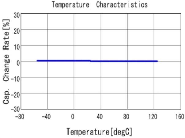
■ GRM2195C1H822JA01 C-Temp. capchange, DCOV, AC1Vrms
