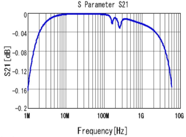
■ GRM2195C1H822JA01 S21 DCOV, 25degC
