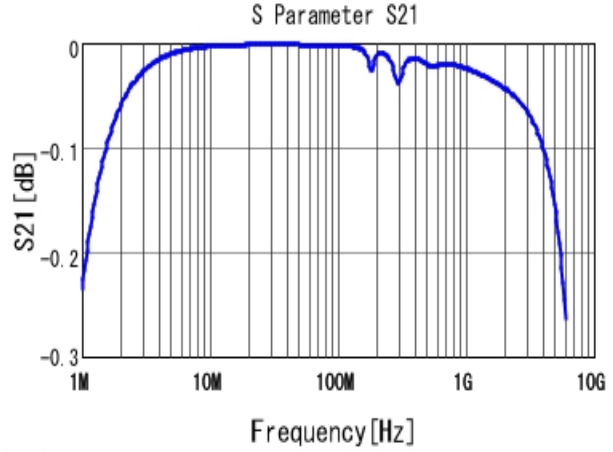
■ GRM2195C1H682JA01 S21 DCOV, 25degC
