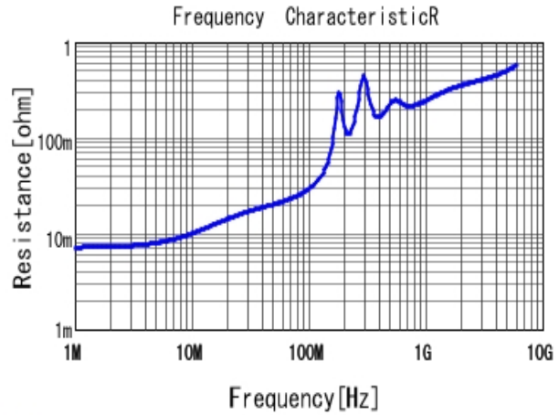
■ GRM2195C1H682JA01 R DCOV, 25degC
