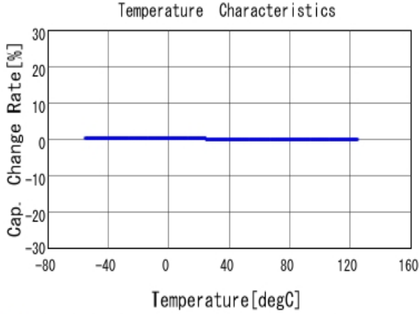
■ GRM2195C1H682JA01 C-Temp. capchange, DCOV, AC1Vrms
