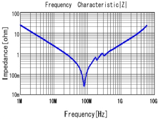
■ GRM2195C1H682JA01 |Z| DCOV, 25degC
