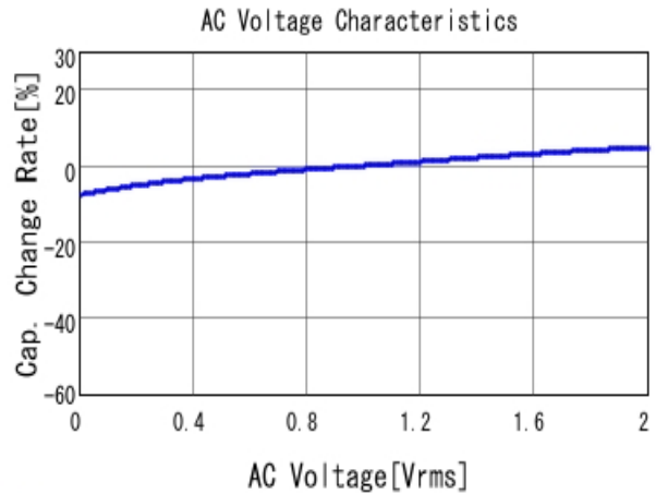
■ GRM033R71E103KE14 C-AC Voltage capchange, DCOV, 25.0d
