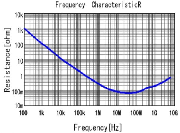
■ GRM033R71E103KE14 R DCOV, 25degC
