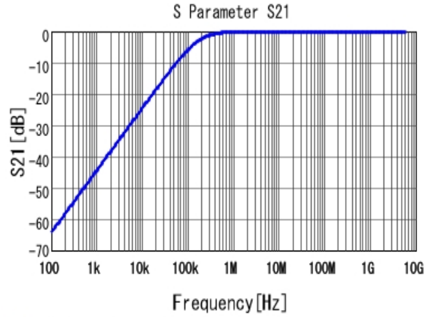
■ GRM033R71E103KE14 S21 DCOV, 25degC
