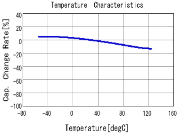
■ GRM033R71E103KE14 C-Temp. capchange, DCO. 0V, AC1.0Vrm
