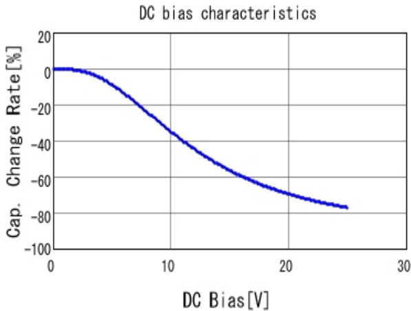
■ GRM033R71E103KE14 C-DC bias capchange, 25.0degC, AC1.
