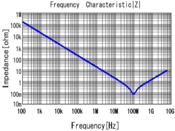
■ GRM033R71E103KE14 |Z| DCOV, 25degC
