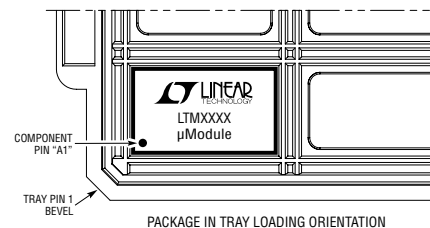
PACKAGE IN TRAY LOADING ORIENTATION BGA 209 0218 REV B
